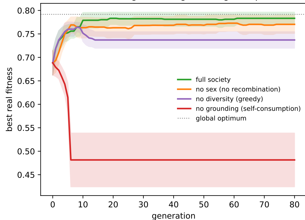
The vertical climb: general capability (full climbs highest; no-grounding collapses)
