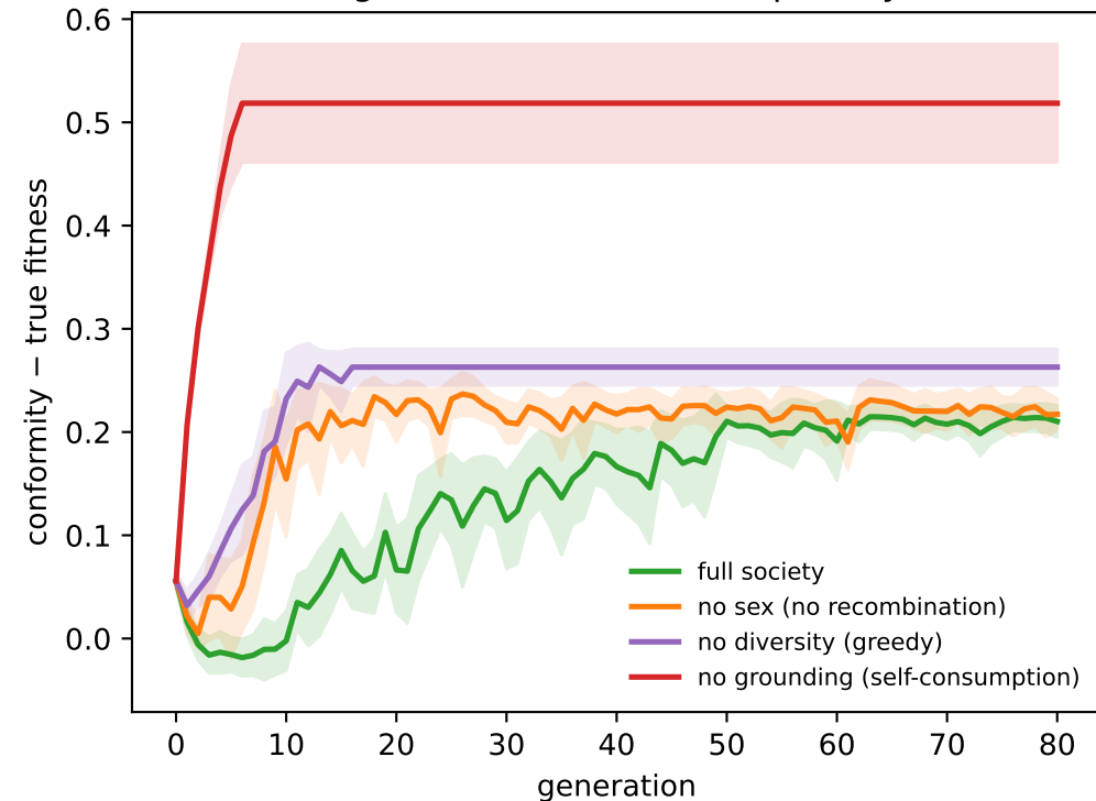
Self-consumption signature: agreement minus real capability
