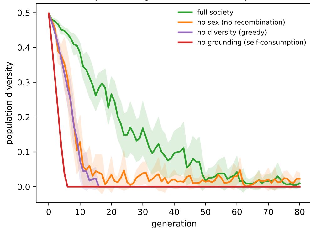
Specialties maintained: diversity during search (full explores longest; ablations collapse fast)
