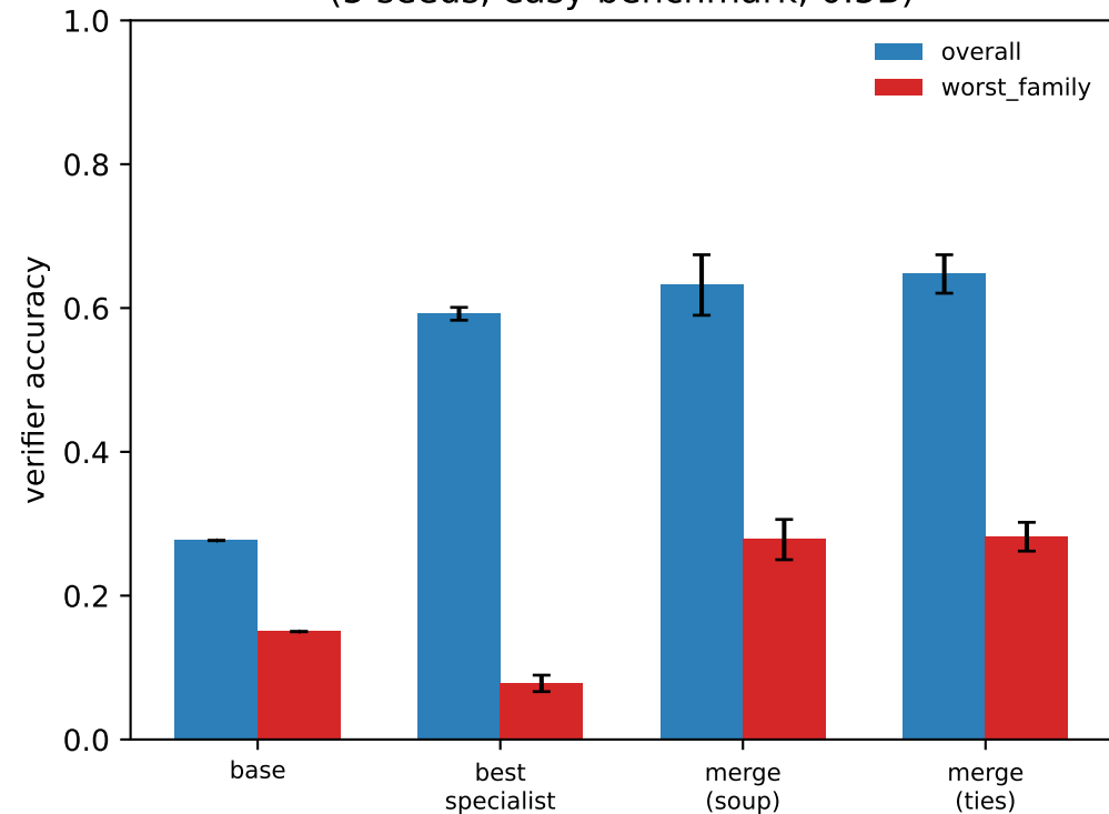
(A) Fisher-Muller with error bars (5 seeds, easy benchmark, 0.5B)
