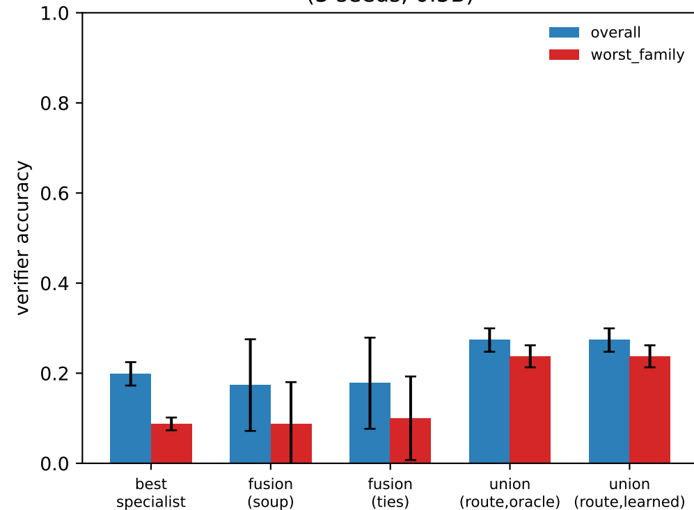
(B) union vs fusion, hard benchmark (3 seeds, 0.5B)
