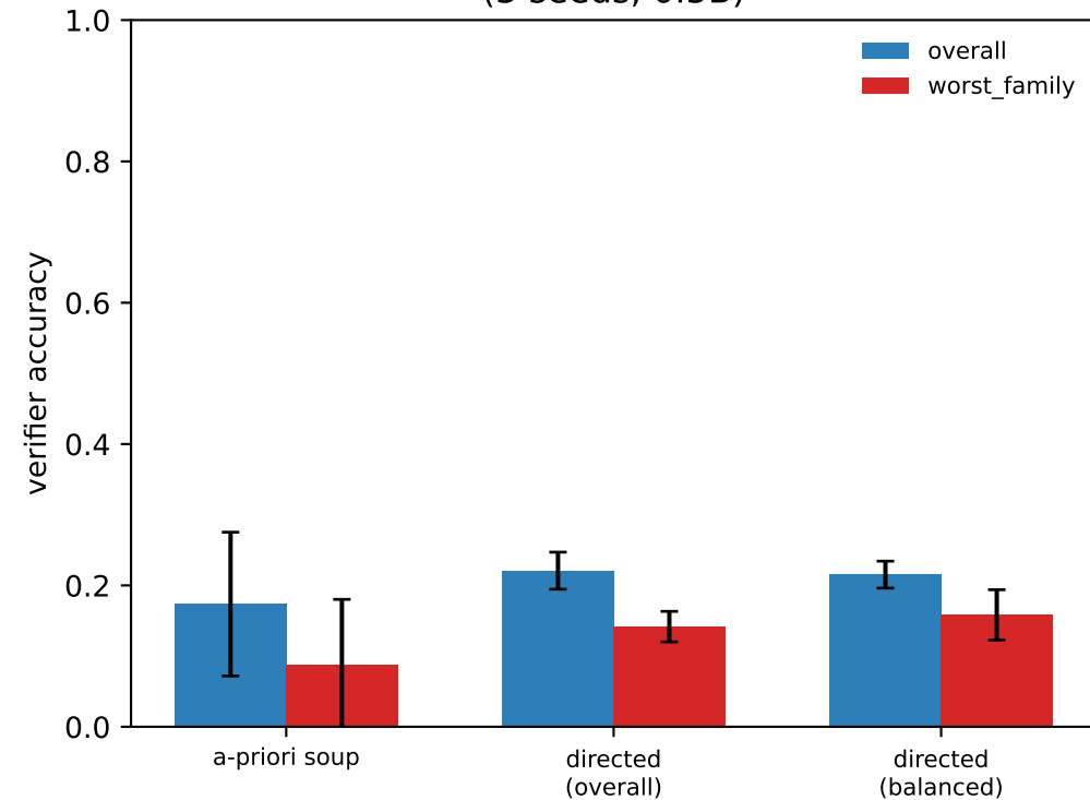
(C) directed offspring selection, hard (3 seeds, 0.5B)
