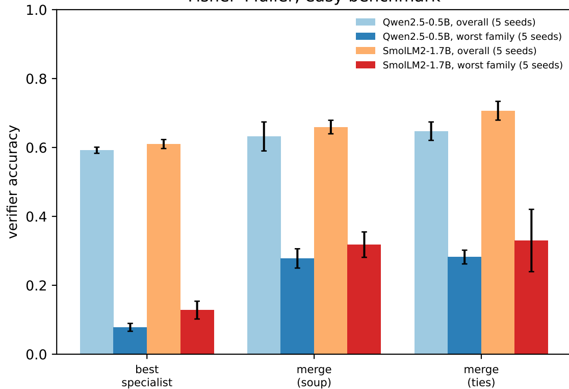
Fisher-Muller, easy benchmark
