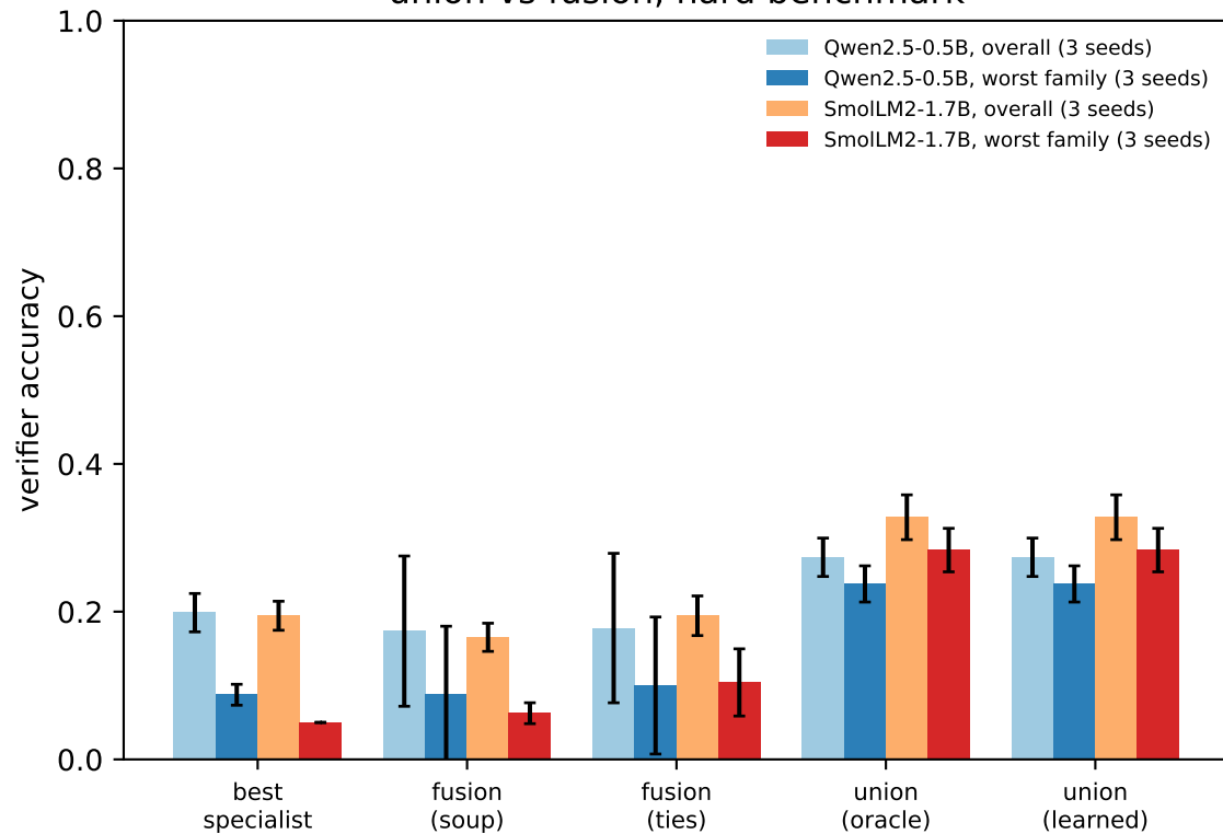
union vs fusion, hard benchmark
